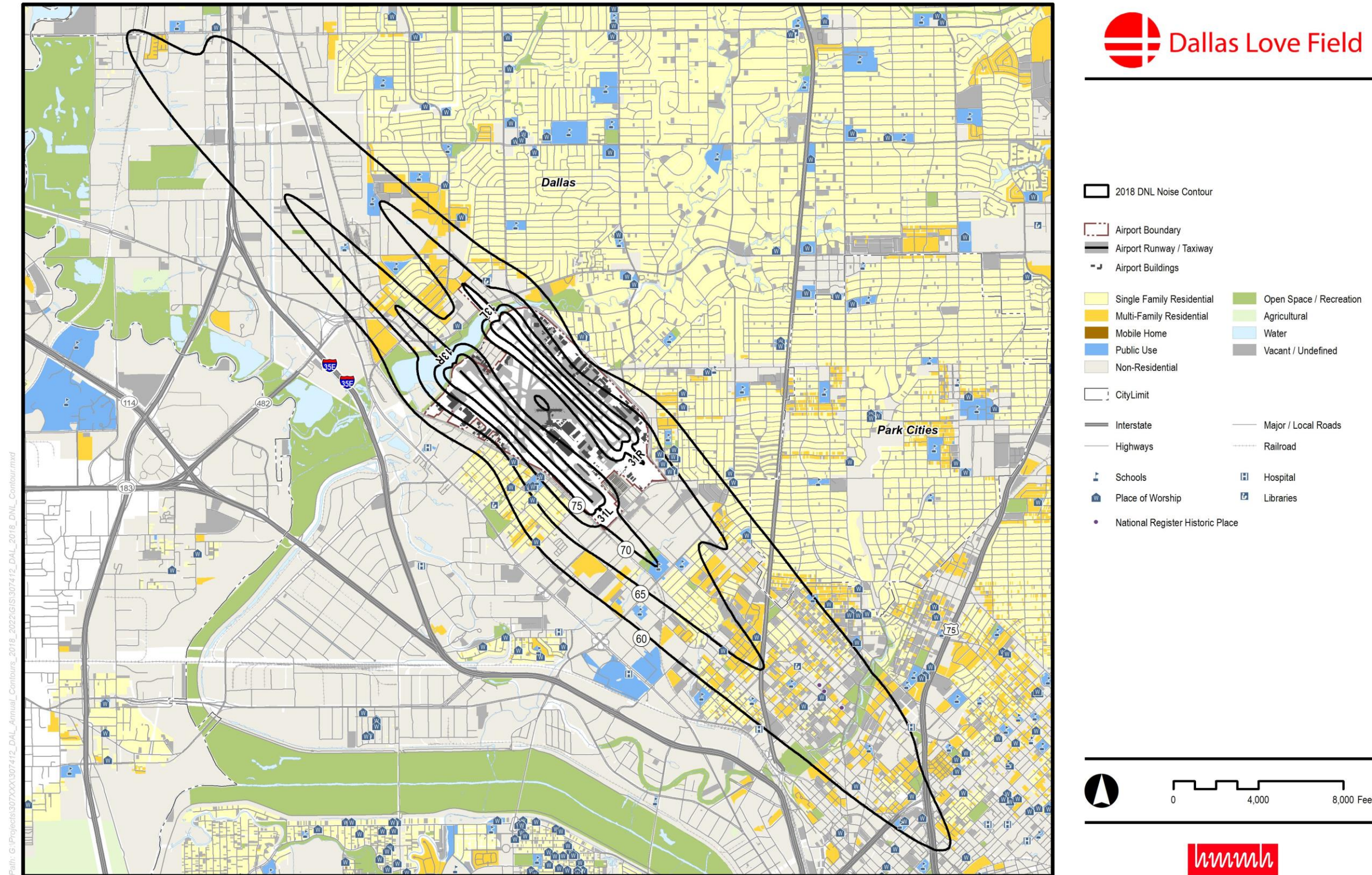
Figure 27. 2018 DNL Contours
