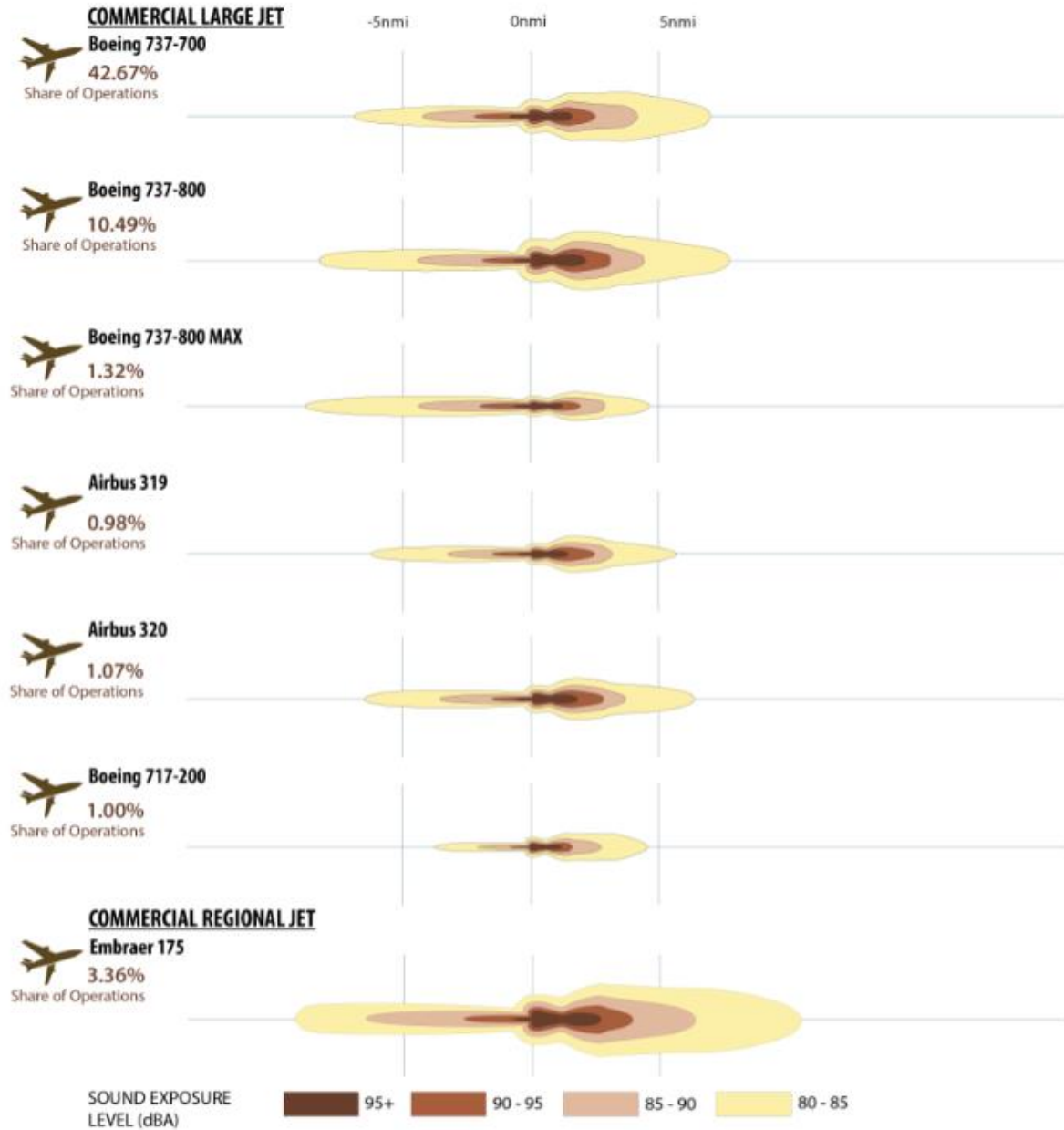
Figure 13. SEL Contours - Commercial Aircraft
