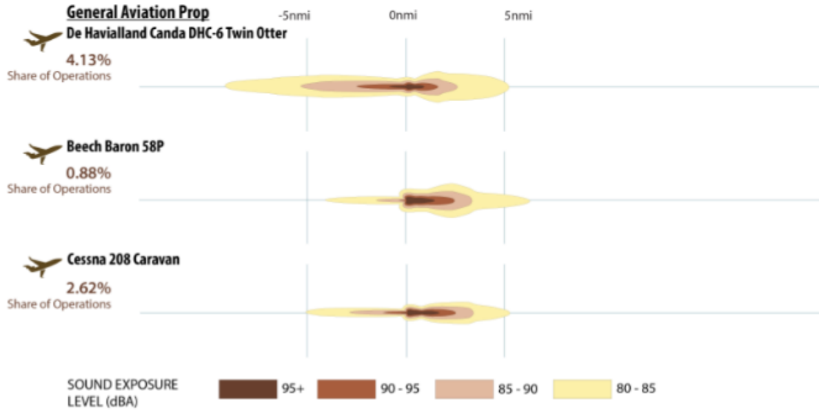
Figure 15. SEL Contours - General Aviation Propellers
