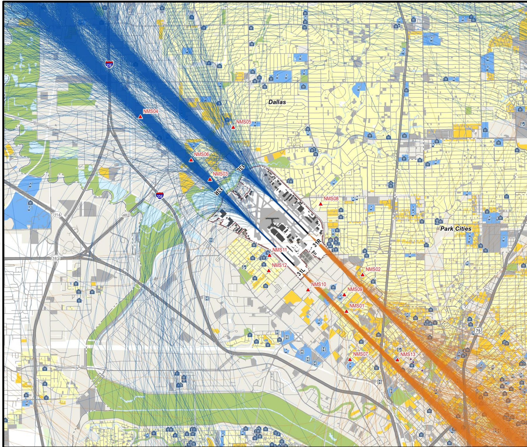
Figure 24. Sample of Modeled North Flow Flight Tracks
