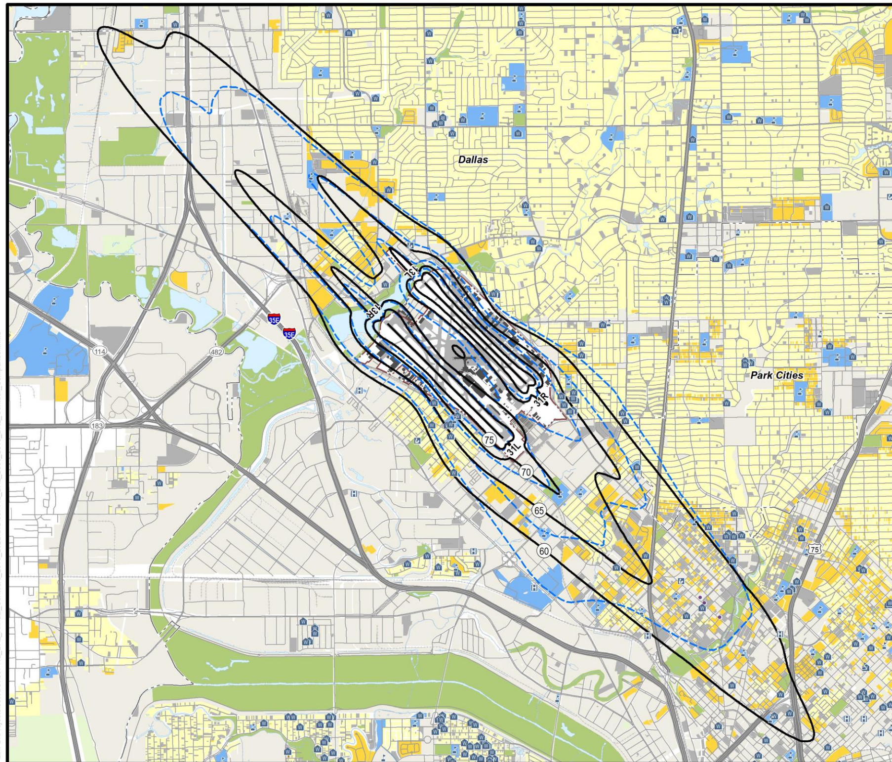
Figure 29. 2018 DNL Contours compared to 2006 DNL Contours
